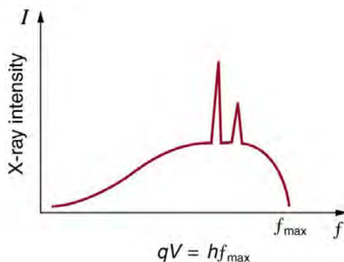
Figure 30.22 X-ray spectrum obtained when energetic electrons strike a material, such as in the anode of a CRT. The smooth part of the spectrum is bremstrahlung radiation, while the peaks are characteristic of the anode material. A different anode material would have characteristic x-ray peaks at different frequencies.
