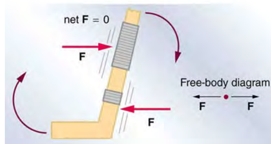
Figure 9.5 The same forces are applied at other points and the stick rotates—in fact, it experiences an accelerated rotation. Here \text{net } F = 0 but the system is not at equilibrium. Hence, the \text{net } F = 0 is a necessary—but not sufficient—condition for achieving equilibrium.
