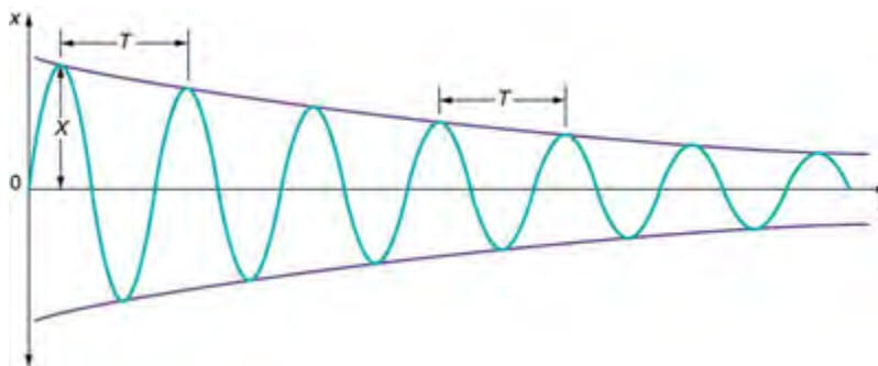
Figure 16.22 In this graph of displacement versus time for a harmonic oscillator with a small amount of damping, the amplitude slowly decreases, but the period and frequency are nearly the same as if the system were completely undamped.
